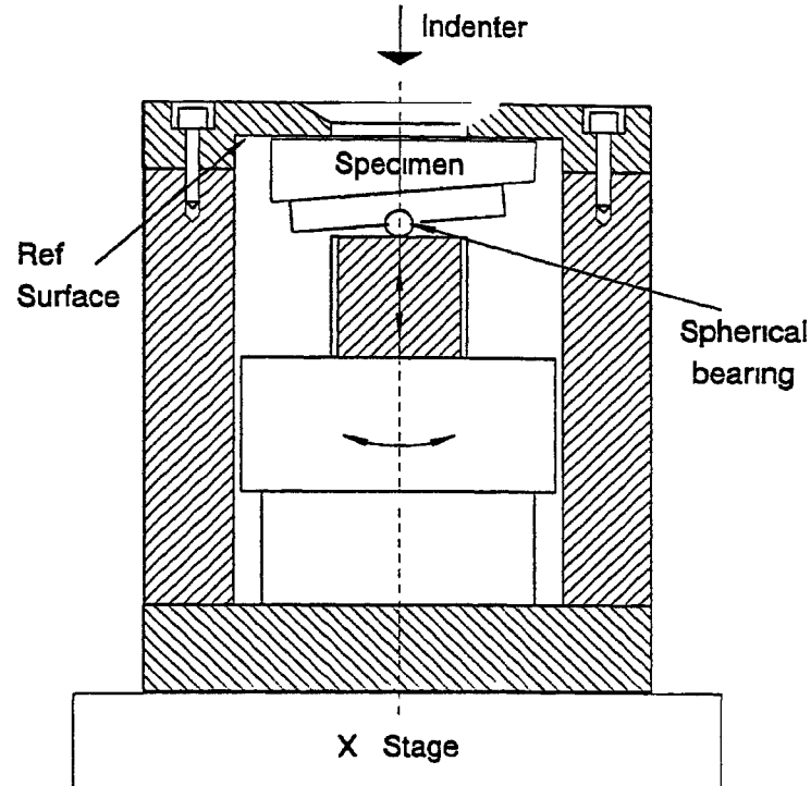
Figure 3 14 Specimen Holder
