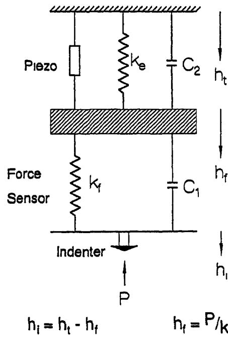
Figure 3 9 Schematic of Force Sensor in relation to the Translator and the Indenter
