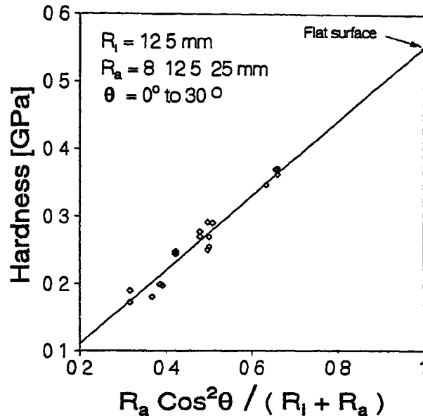
Figure 4.8 Plot of hardness versus R_a \cos^2 \theta / (R_1 + R_a) , \diamond experimental, — eqn(8)
