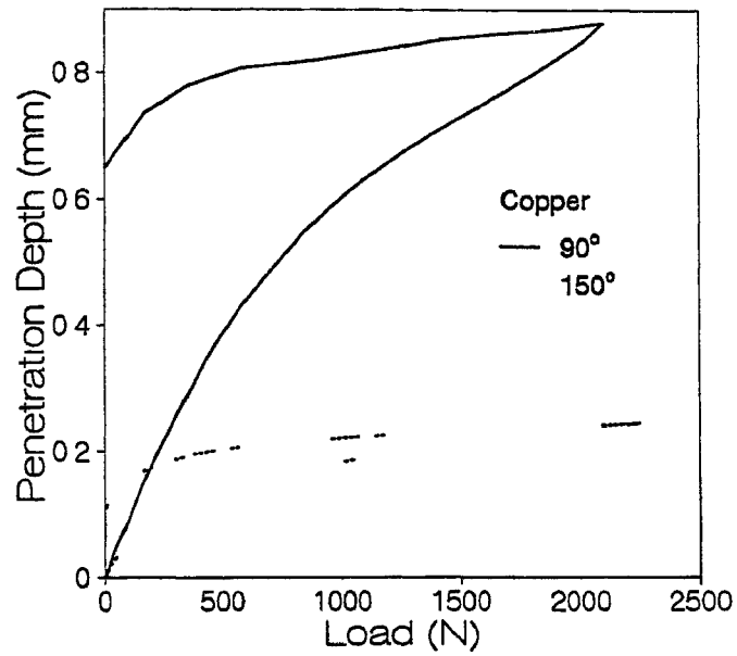
Figure 2.2 Displacement - Load Characteristics of Copper
