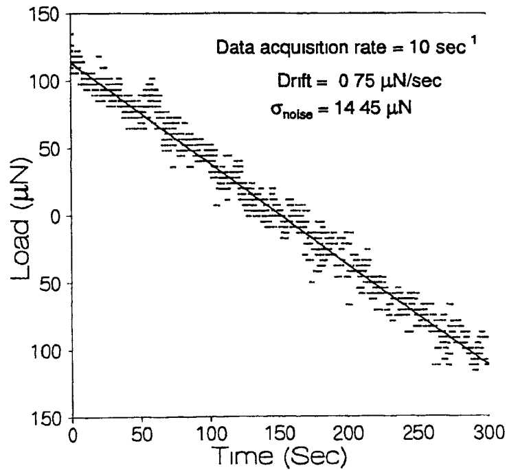
Figure 3 17 Force sensor output
