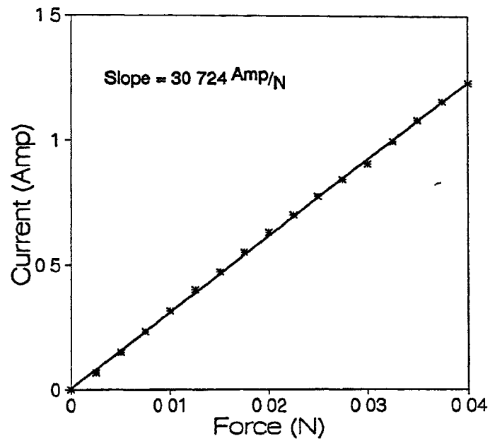
Figure 3 19 Calibration curve for the coil and the magnet
