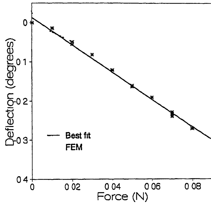
Figure 3.3 Calibration of the Flexure Hinge
