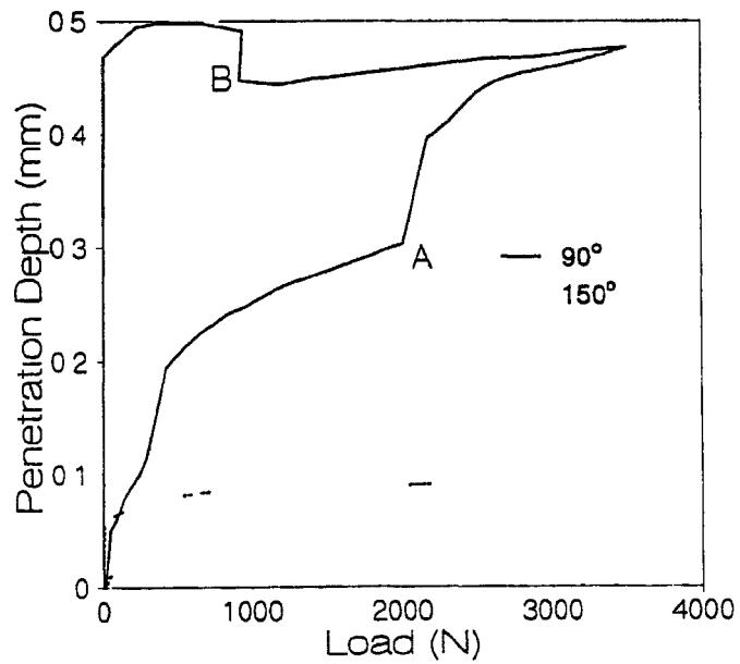
Figure 2.3 Displacement - Load Characteristics of Alumina
