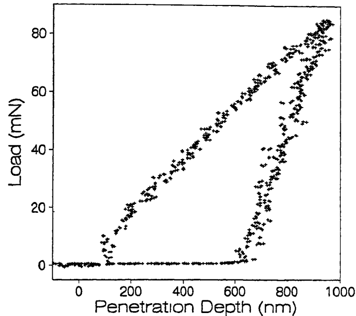
Figure 3 21 Typical Load-Displacement Curve
