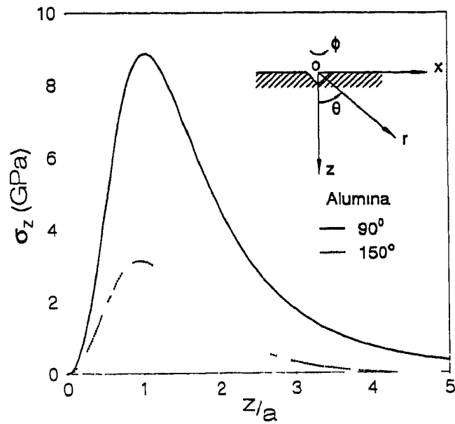
Figure 2 12 Estimate of \sigma_z generated by indentation of alumina at x = a
