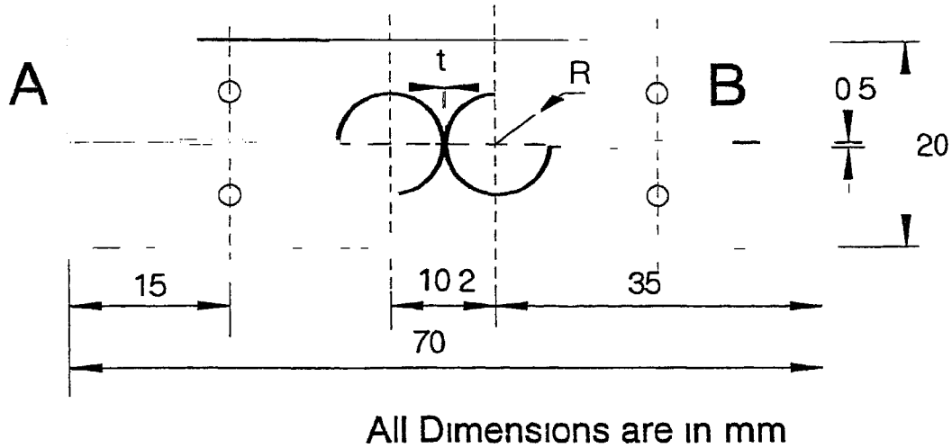
Figure 3.2 Flexure Hinge
