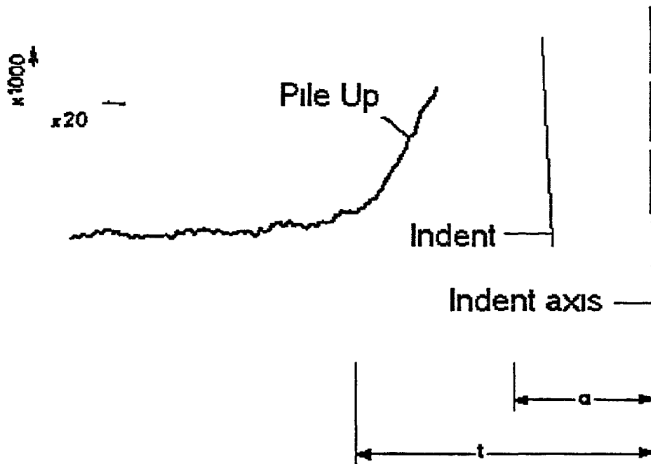
Figure 2.9 Radial surface profile of a pile up generated by 150^\circ indentation of copper
