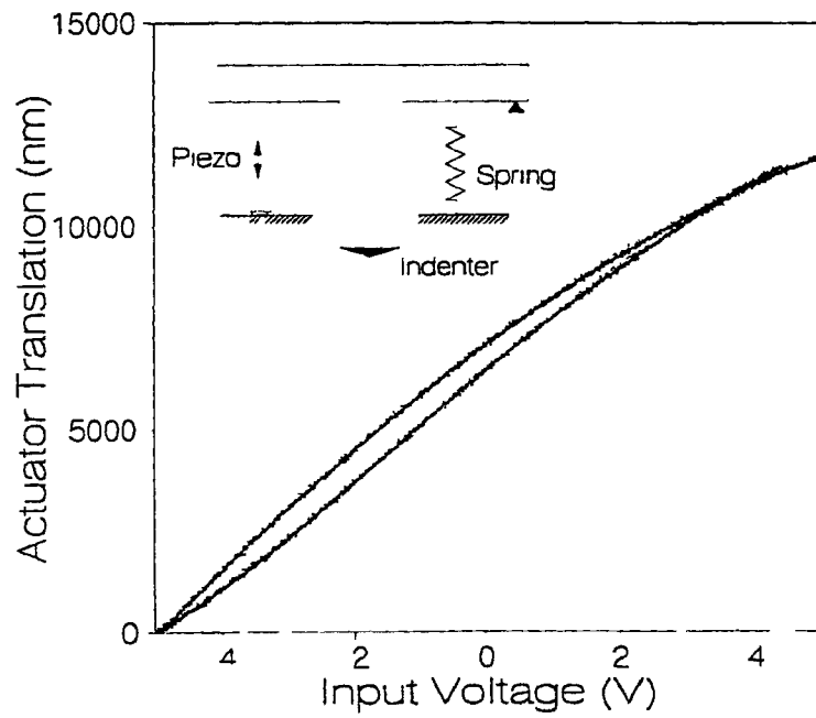
Figure 3 7 Response of the piezo translator in operating condition
