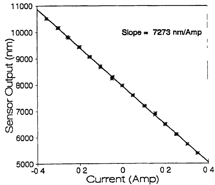
Figure 3 20 Calibration curve for force sensor
