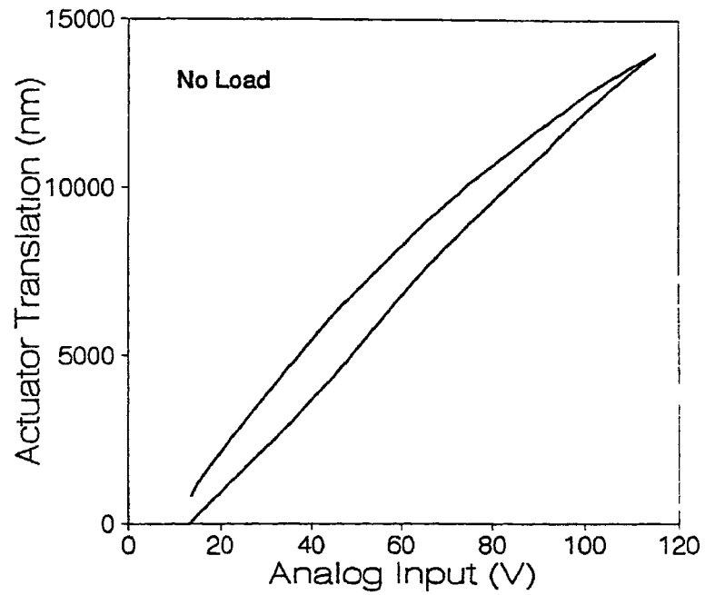
Figure 3 6 Response of the piezo translator
