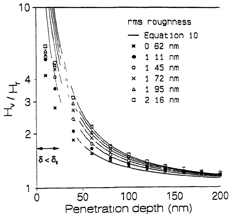
Figure 6 3 Mean hardness variation for different roughness
