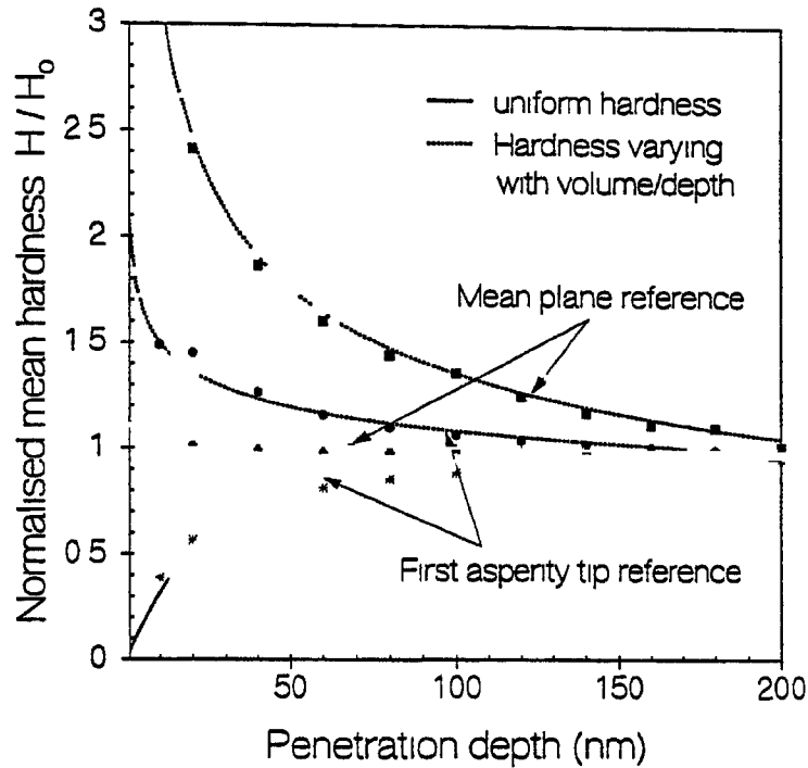
Figure 6.2 Mean hardness variation with penetration
