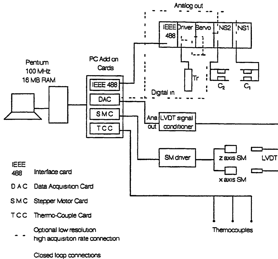
Figure 3 15 Schematic of the Electronics
