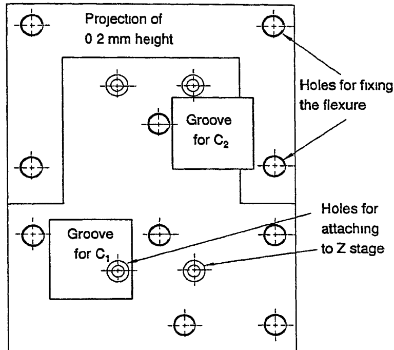
Figure 3 13 Buffer Plate
