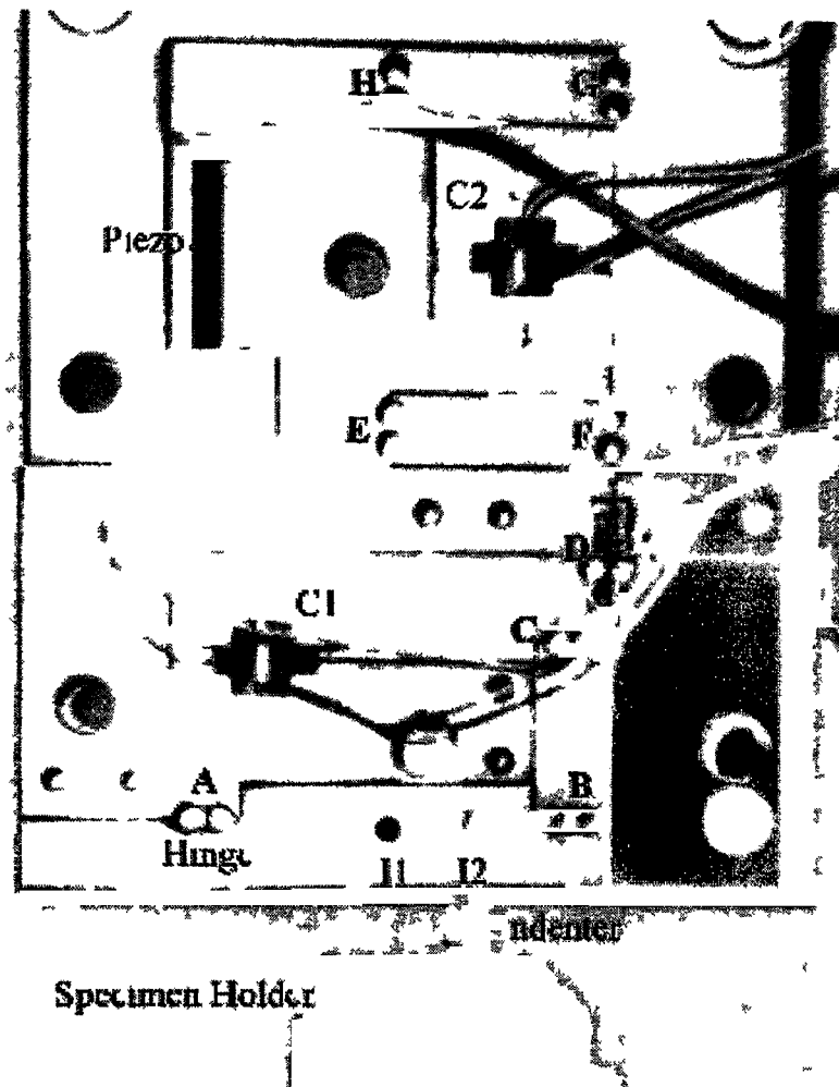
Figure 3 11 Flexure
