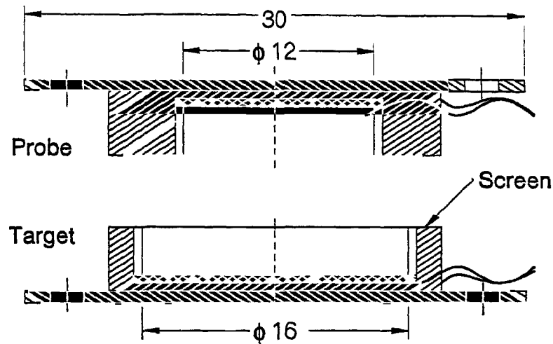
Figure 3.8 Schematic of Displacement Sensors
