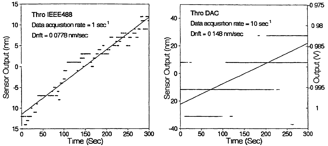
Figure 3 16 Displacement sensor output
