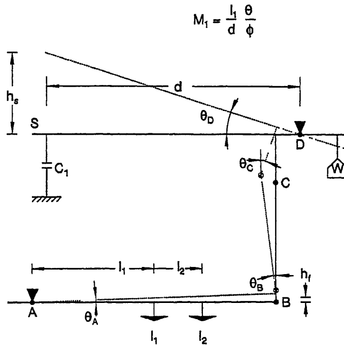
Figure 3 10 Schematic of the Force Sensor
