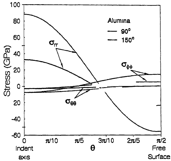
Figure 2 11 Estimates of stresses generated by indentation of alumina
