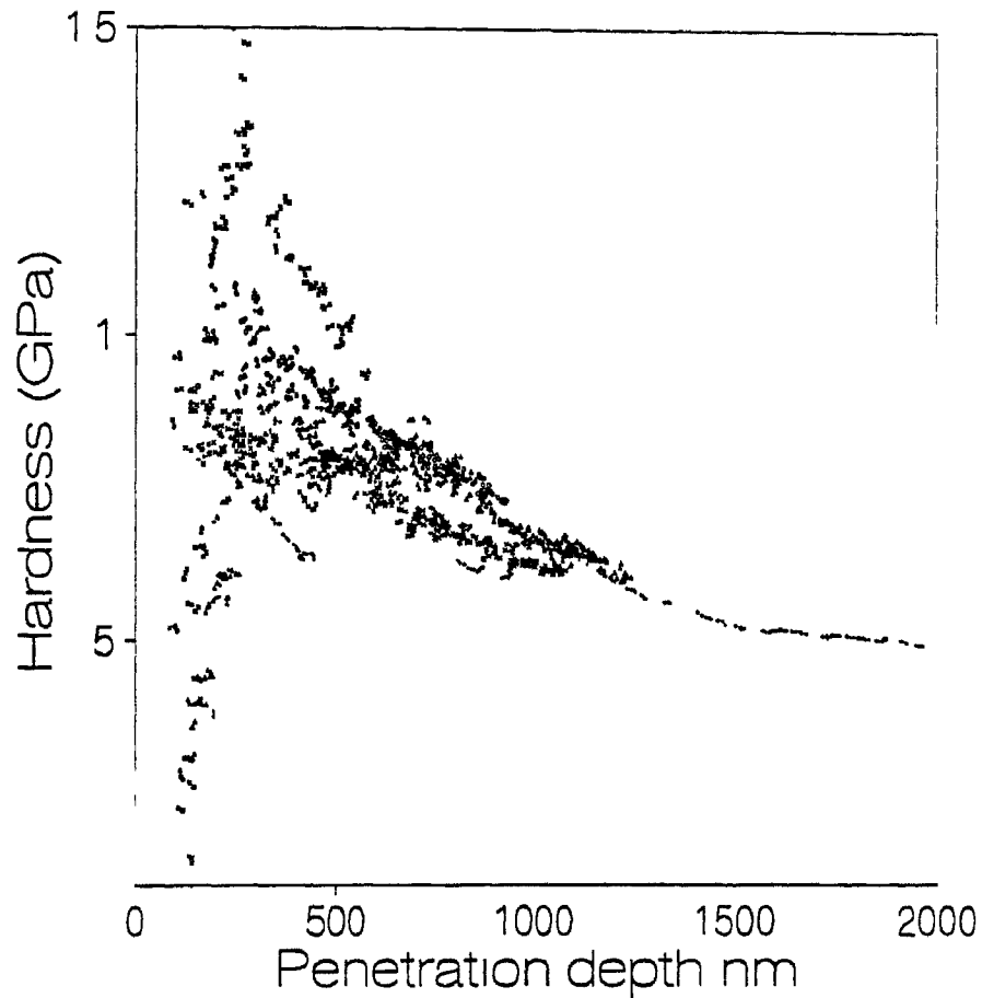
Figure 3 24 Variation of Hardness with penetration depth
