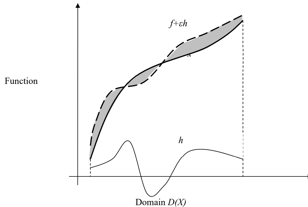
Figure 1. Pictorial depiction of variation \epsilon h of a function f
